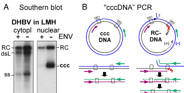
Figure 5 Direct versus indirect detection of covalently closed circular (ccc)DNA. (A) Southern blotting. Vectors for wild-type (+ENV) and envelope-deficient (-ENV) duck HBV (DHBV) were transfected into the avian hepatoma cell line LMH. Viral DNAs from cytoplasmic nucleocapsids (cytopl) and in nuclear DNA were detected using a ^{32} P-labeled DHBV DNA probe; nuclear DNAs were treated with Dpn I to digest bacterially derived transfected plasmid, and with Plasmid-Safe nuclease that degrades linear but not circular DNA; relaxed circular (RC)-DNA with a nearly completed (+)-strand is not degraded. Note (i) the characteristically distinct mobility of cccDNA from all other viral DNA forms and (ii) the drastically enhanced cccDNA levels generated from the envelope-deficient DHBV. (B) 'cccDNA-specific' PCR. Primers (purple and green arrows) are chosen to span the region containing the gap in the (+)-strand and the nick in the (-)-strand of RC-DNA. cccDNA provides a continuous template for exponential amplification. On RC-DNA, linear extension of the individual primers generates shorter but overlapping products that can anneal to each other and subsequently form an identical amplicon as that from cccDNA.
